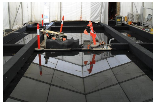
Flood Testing
